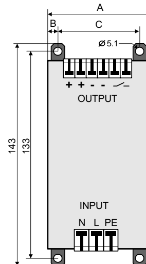
Fig. 2-2 Mounting dimensions
